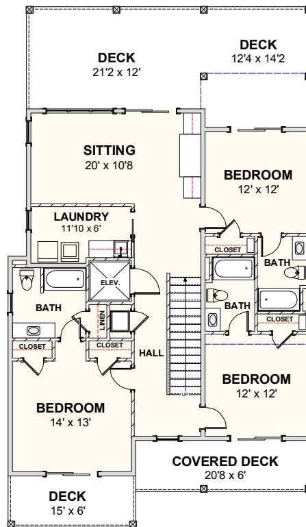
2ND FLOOR - FLOOR PLAN
