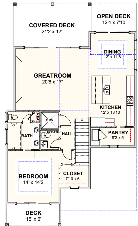
3RD FLOOR - FLOOR PLAN
